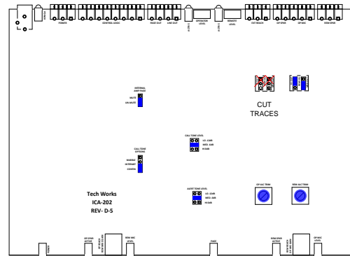
ICA-202D Remote Unit Jumpers
