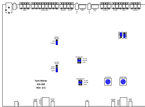
ICA-202D Operator Unit Jumpers
